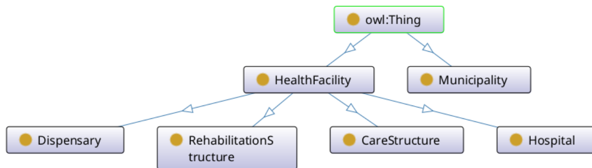
Figure 2: Ontology Language Definition
